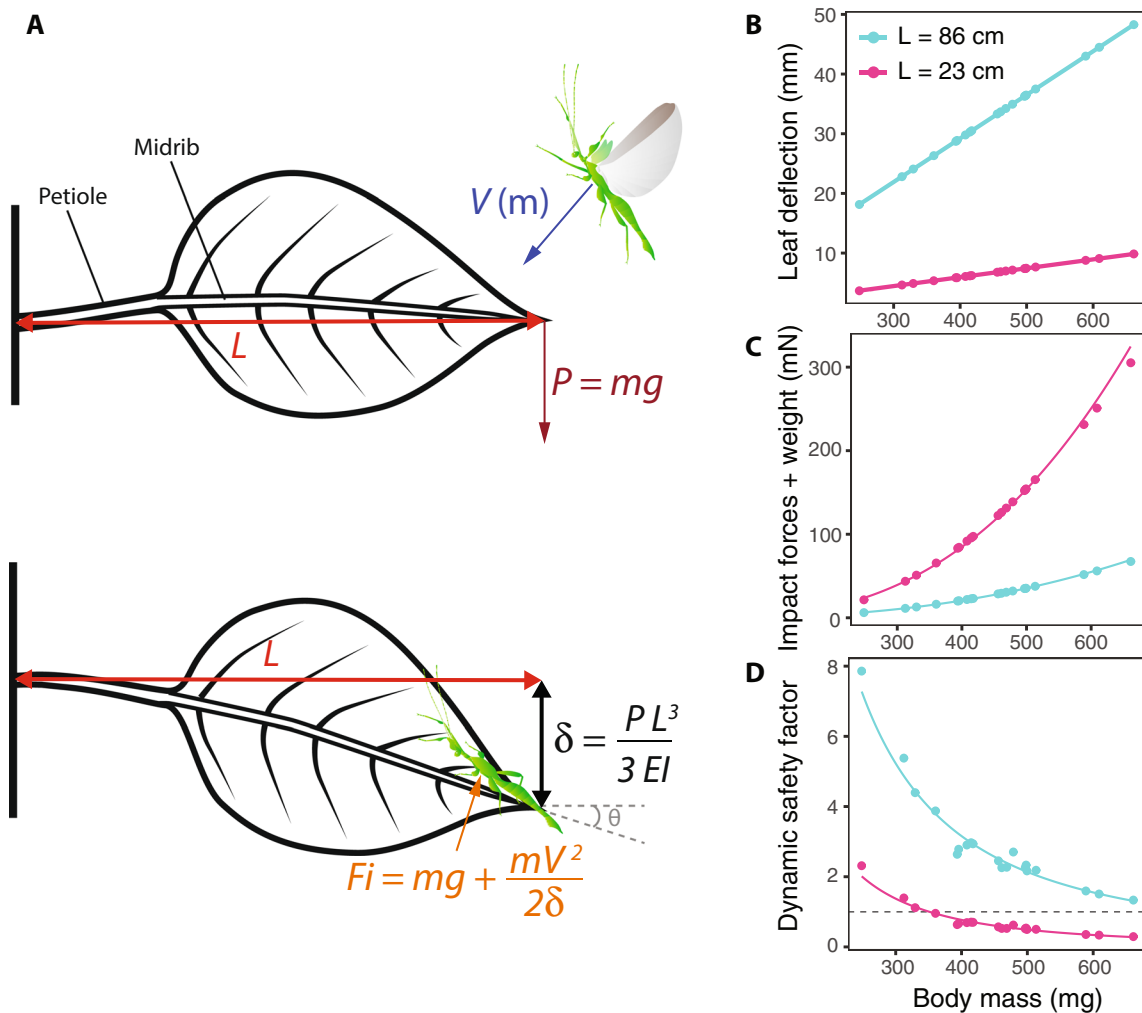
Fig. 4 Landing model calculations and predictions. A Diagram of a male leaf insect landing on a leaf, including calculations used to estimate impact forces ( F_i ) and dynamic safety factors ( SF_{dynamic} )—i.e., the ratio of frictional attachment forces and F_i . The male lands with a landing velocity V which depends on the body mass of the insect ( m ). The terminal load on the leaf ( P ) will be equal to the weight of the insect—i.e., body mass ( m ) multiplied by the acceleration due to gravity ( g ). The subsequent deflection of the leaf ( \delta ) depends on P , the length of the leaf ( L ) and the leaf flexural stiffness ( EI ). The impact force experienced by the male leaf insect ( F_i ) will be determined by P , the kinetic energy of the insect ( mV^2/2 ) and \delta . See the text for more detailed information. Predicted relationships between male body mass ( m ) and \delta ( B ), F_i ( C ) and SF_{dynamic} ( D ). Predictions for large leaves ( L = 86 \text{ cm} ) are represented in blue, small leaves ( L = 23 \text{ cm} ) in pink. The dashed line in ( D ) represents a safety factor of one
